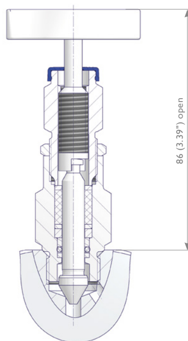
Picture shows ISO FE Type 1
