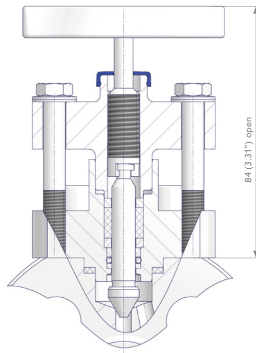
Picture shows ISO FE Type 1
